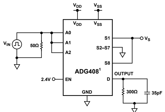
Figure 23. Break-Before-Make Delay, t_{\text{OPEN}}
