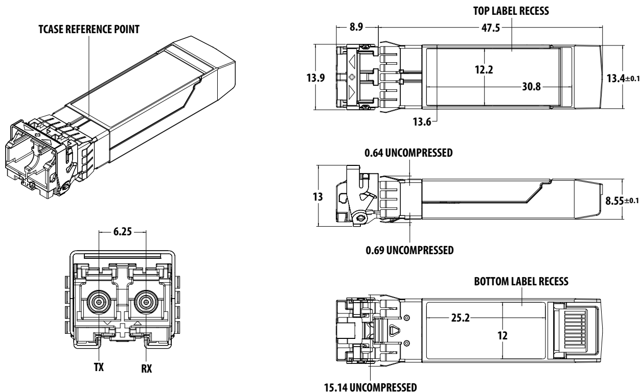
Figure 5. Module drawing
