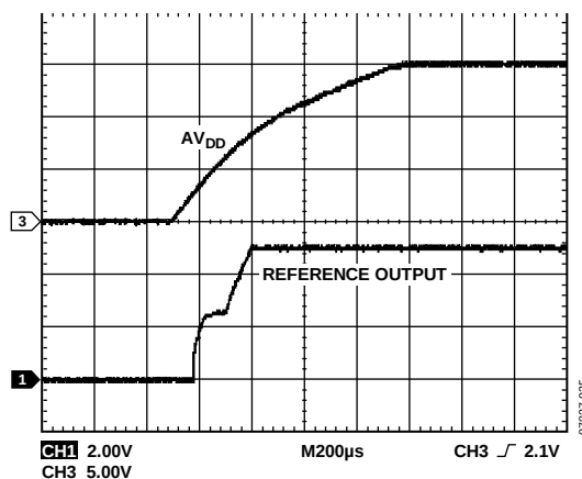
Figure 28. Reference Turn-on Transient
