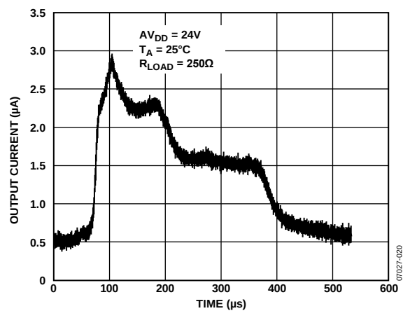
Figure 23. Output Current vs. Time on Power-Up
