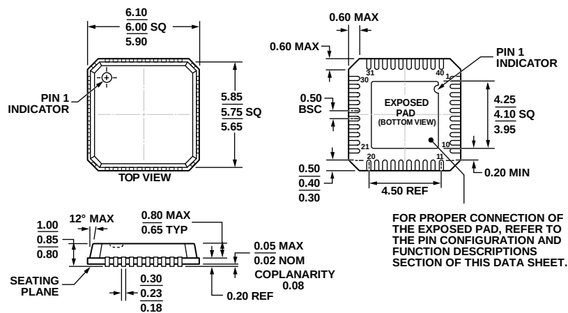
Figure 57. 40-Lead Lead Frame Chip Scale Package [LFCSP_VQ] 6 mm x 6 mm Body, Very Thin Quad (CP-40-1)
