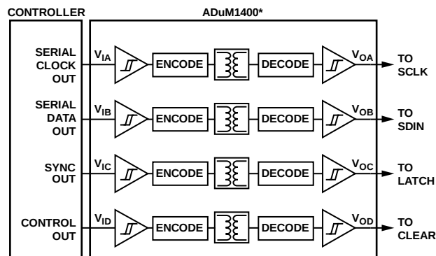
Figure 52. Isolated Interface
