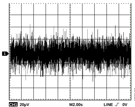
Figure 30. Reference Noise (100 kHz Bandwidth)
