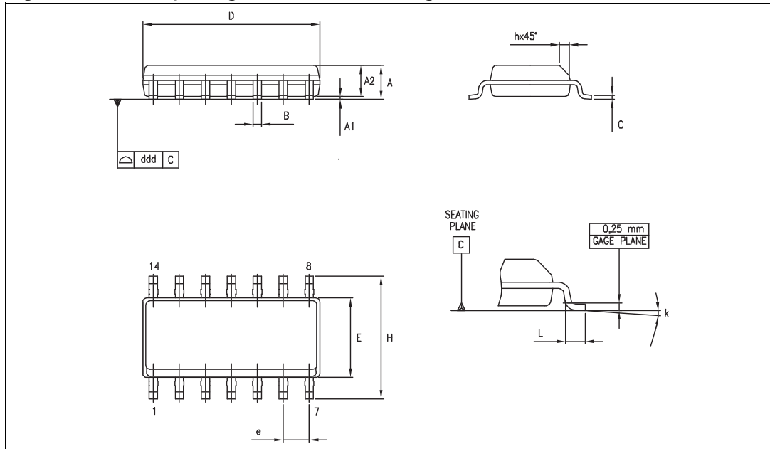
Figure 34. SO-14 package mechanical drawing
