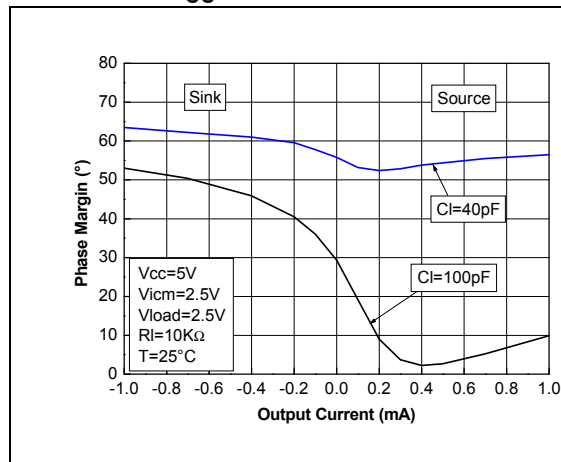
Figure 12. Phase margin vs. output current at V_{CC} = 5 \text{ V}
