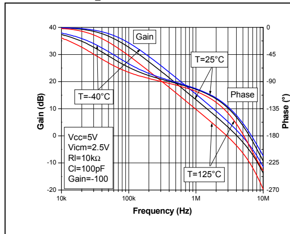
Figure 10. Voltage gain and phase with C_L = 100 \text{ pF}
