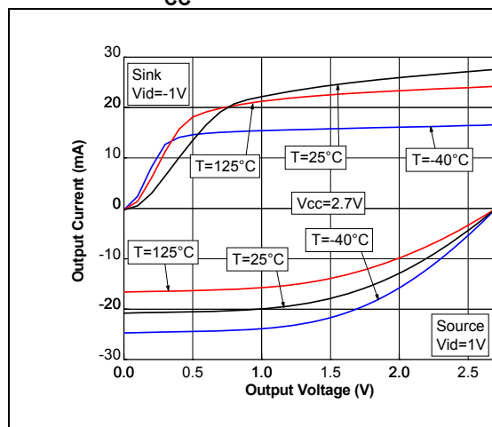
Figure 6. Output current vs. output voltage at V_{CC} = 2.7V
