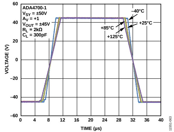
Figure 53. Large Signal Transient Response, V_{SV} = \pm 50\text{ V}
