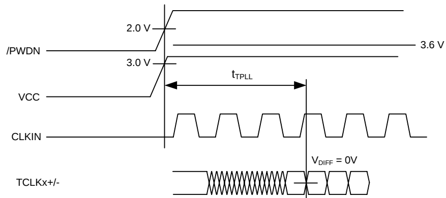
Phase Lock Loop Set Time
