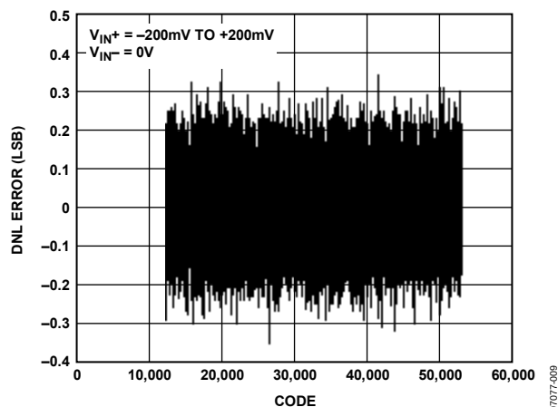
Figure 11. Typical DNL, \pm 200 mV Range (Using \text{Sinc}^3 Filter, 256 Decimation Rate)
