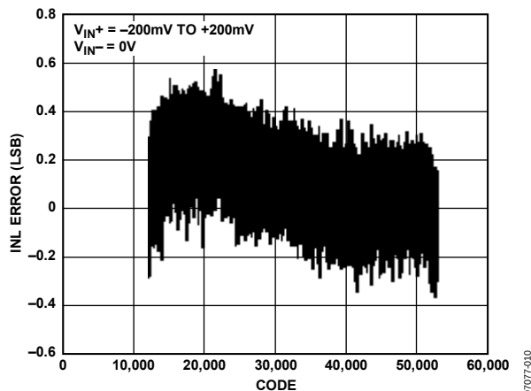
Figure 12. Typical INL, \pm 200 mV Range (Using \text{Sinc}^3 Filter, 256 Decimation Rate)
