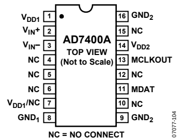
Figure 6. 16-Lead SOIC Pin Configuration
