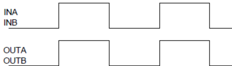
Figure 3. Timing Diagram
