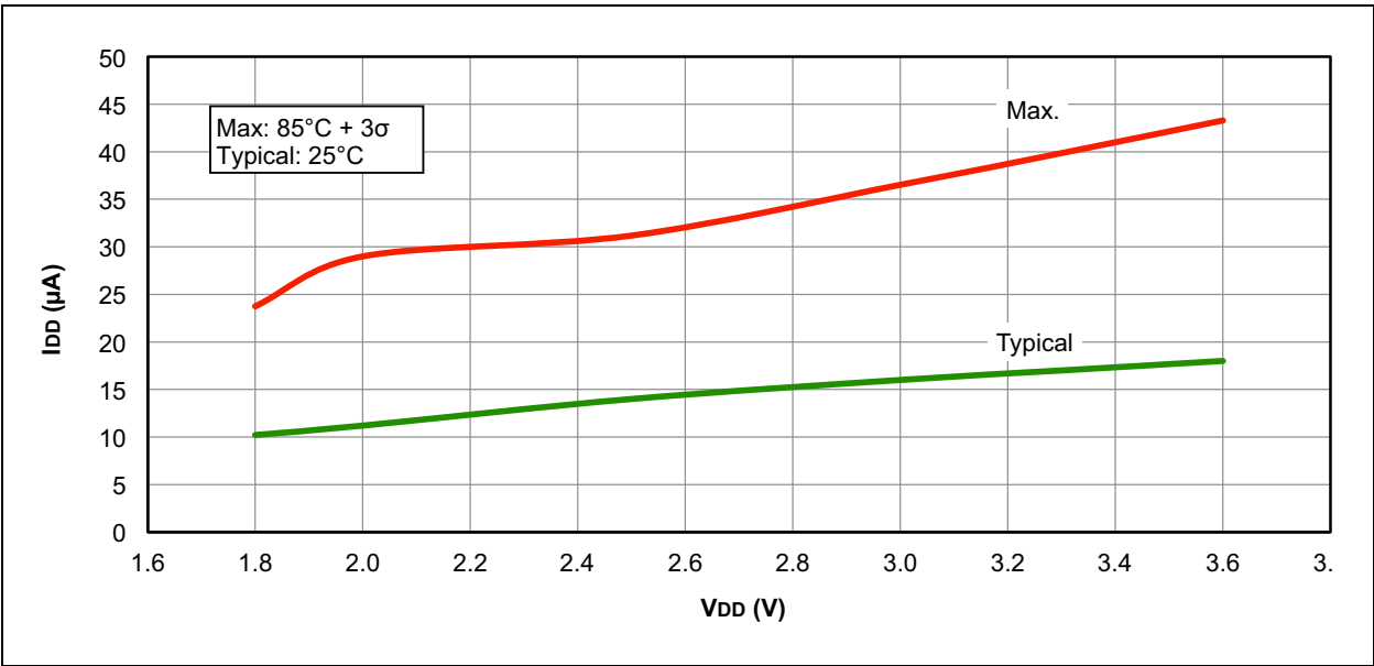
FIGURE 22-2: I DD , EC OSCILLATOR, LOW-POWER MODE, F osc = 500 kHz
