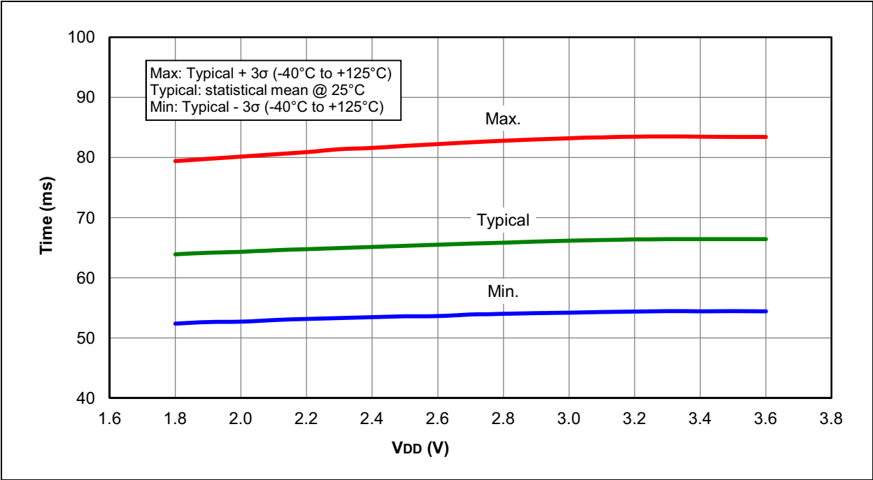
FIGURE 22-20: PWRT PERIOD
