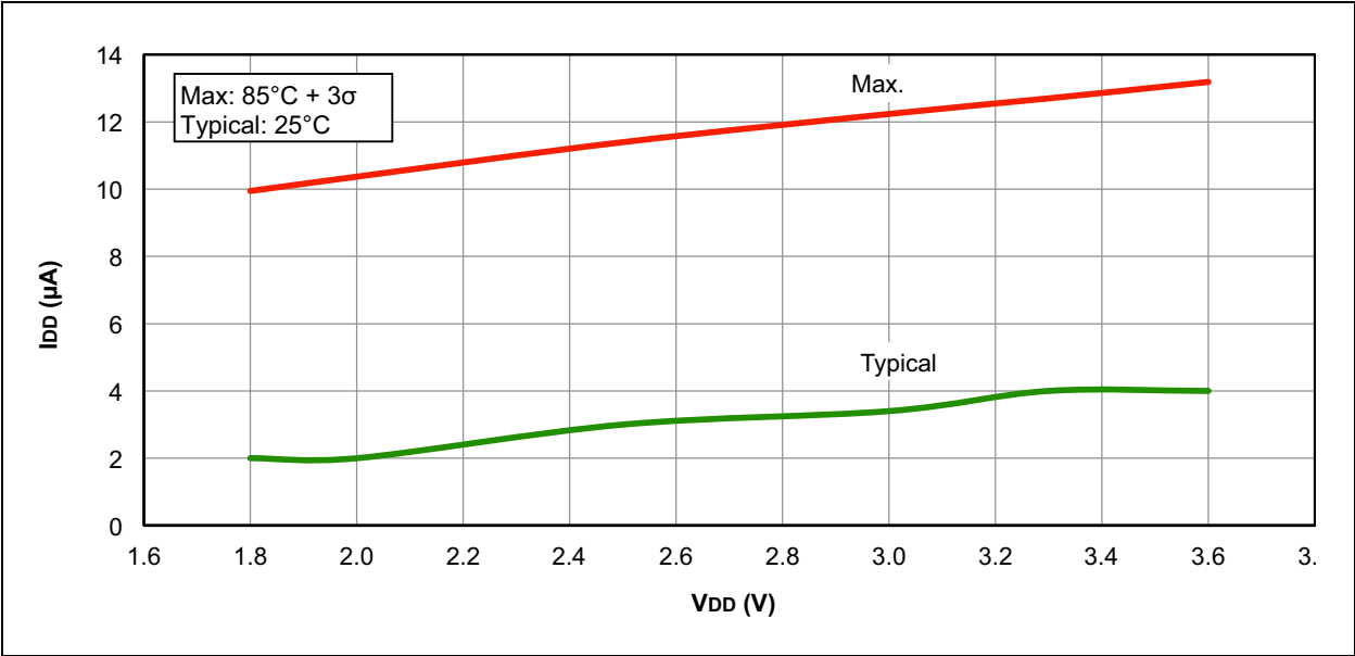
FIGURE 22-1: I DD , EC OSCILLATOR, LOW-POWER MODE, F osc = 32 kHz
