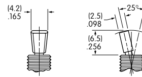
E2 .256" (6.5mm) Flatted
