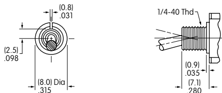
A1 .280" (7.1mm) Threaded with Keyway
