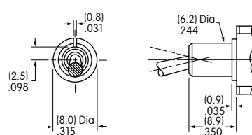
S2 .350" (8.9mm) Smooth with Keyway
