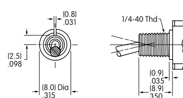
S1 .350" (8.9mm) Threaded with Keyway
