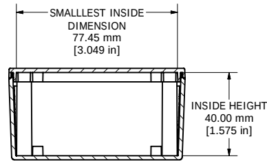
SECTION L-L
