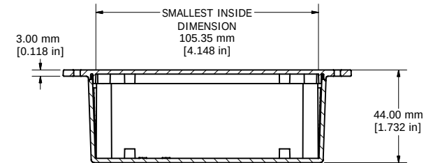
SECTION M-M
