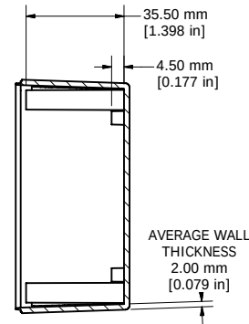
SECTION K-K
