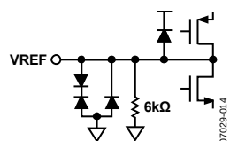
Figure 32. Equivalent VREF Circuit
