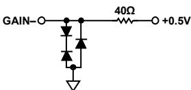
Figure 34. Equivalent GAIN- Input Circuit
