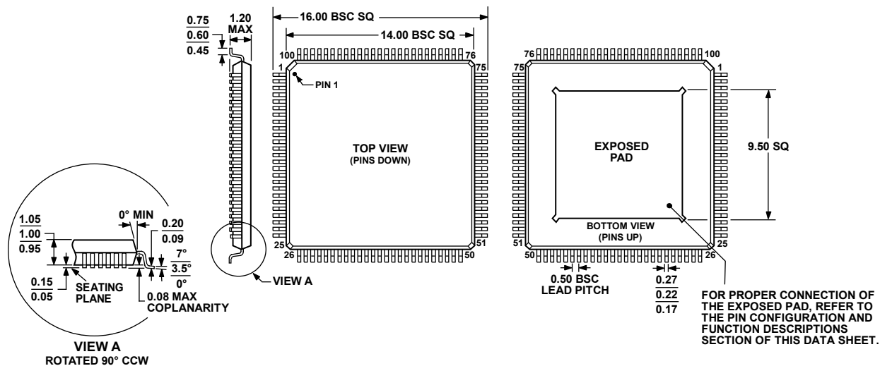
Figure 70. 100-Lead Thin Quad Flat Package, Exposed Pad [TQFP_EP] (SV-100-3)
