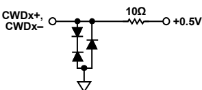
Figure 35. Equivalent CWDx± Output Circuit
