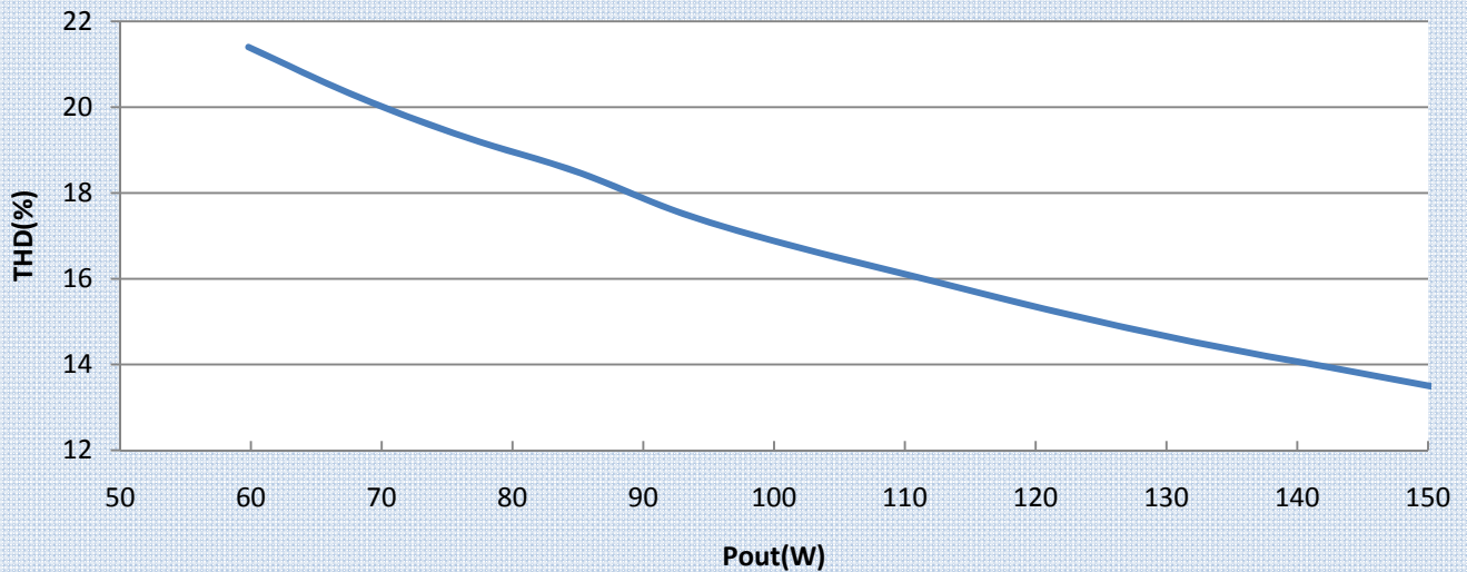
THD VS Pout @ TC 80C @Vin-230V
