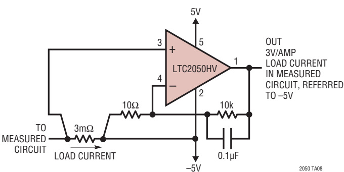
Low Side Power Supply Current Sensing
