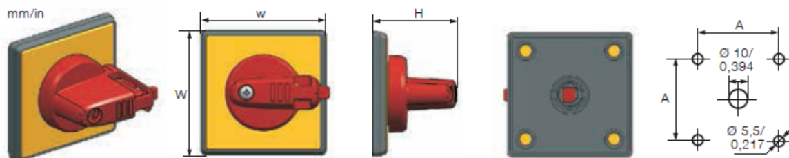
Padlockable nose handle
