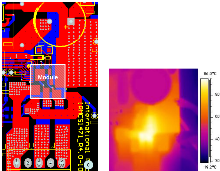
Figure 7: PCB layout example and corresponding thermal image (6kHz, 2P, 2oz, \Delta T_{\text{ca}}=70^\circ\text{C} , V_+ = 150\text{V} , I_u = 870\text{mA}_{\text{rms}} , P_o = 148\text{W} )
