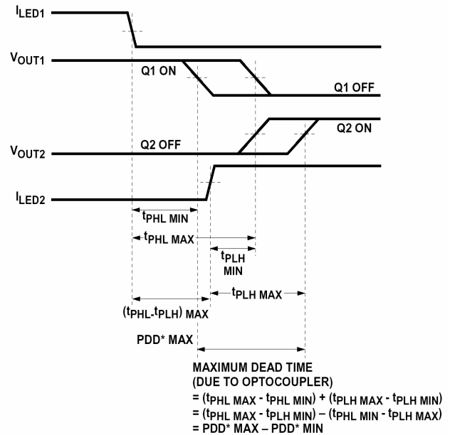
Figure 27. Waveforms for Dead Time.
