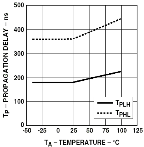
Figure 12. Propagation Delay vs. Temperature.
