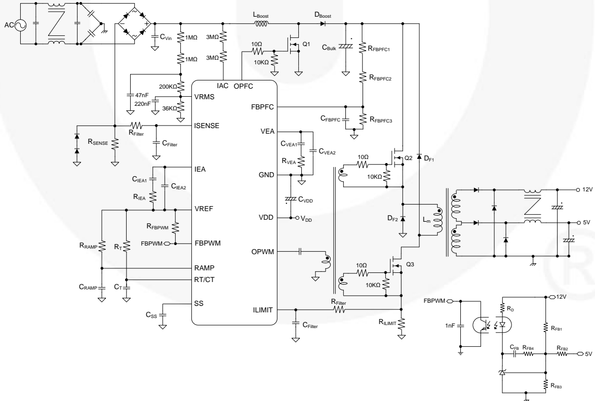
Figure 3. Voltage Mode
