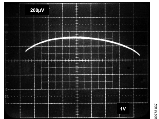
Figure 37. Gain Nonlinearity, G = -1 (50 ppm/DIV)
