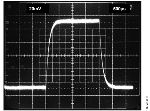
Figure 36. Small Signal Pulse Response, G = 1000 , R_L = 10 \text{ k}\Omega , C_L = 100 \text{ pF}
