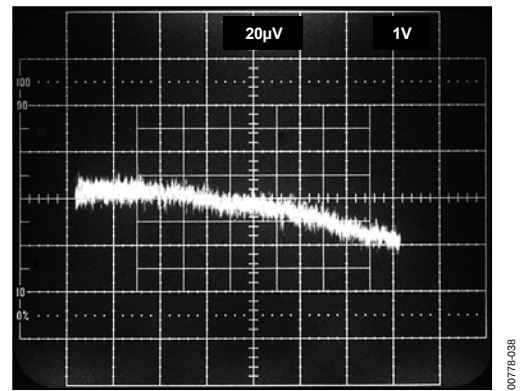
Figure 38. Gain Nonlinearity, G = -10 (6 ppm/DIV)
