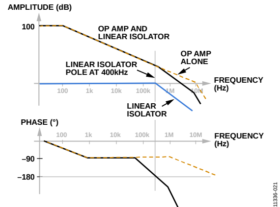
Figure 30. Bode Plot 1: Op Amp and Linear Isolator
