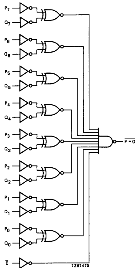
Fig.5 Logic diagram.
