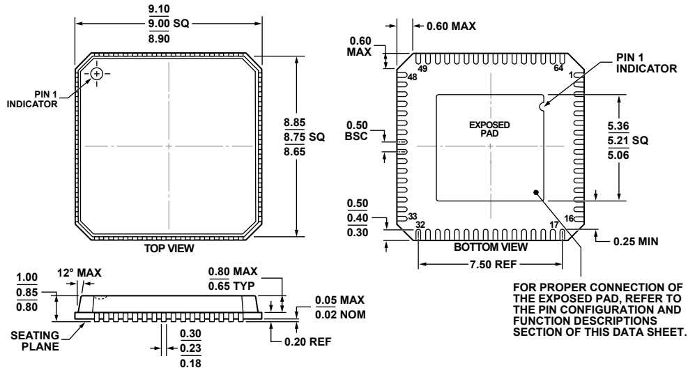
Figure 60. 64-Lead Lead Frame Chip Scale Package [LFCSP_VQ]
