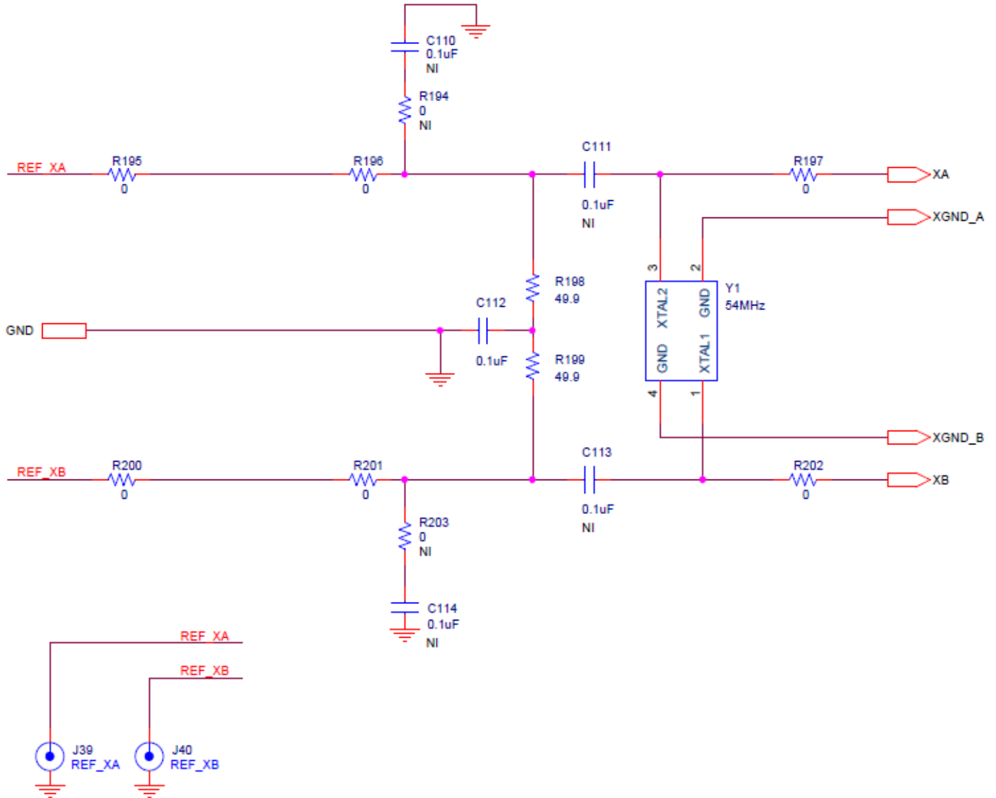
Figure 4.1. External Reference Input Circuit
