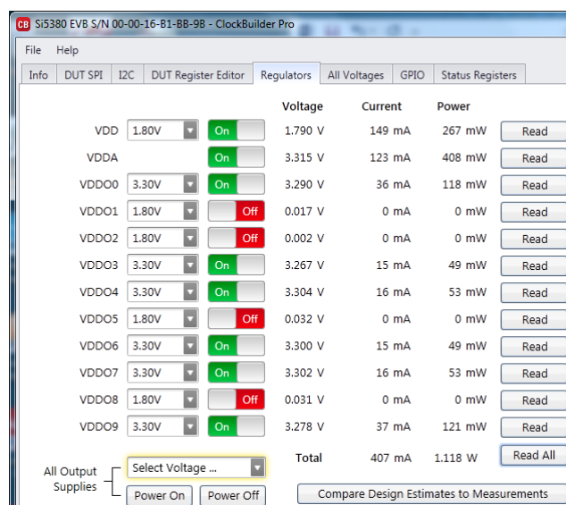
Figure 6.5. EVB GUI
