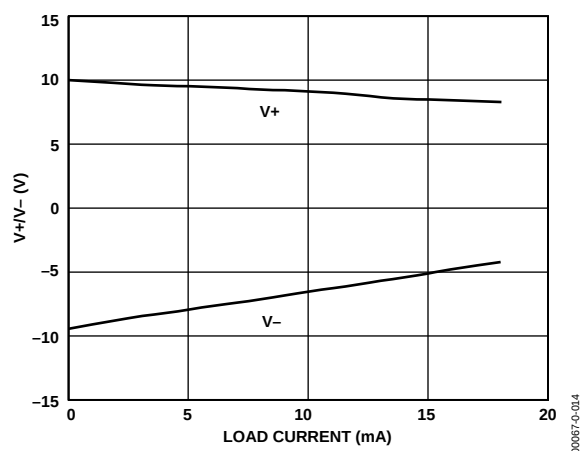
Figure 12. Charge Pump V+, V- vs. Load Current
