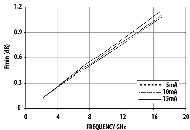
Figure 10. NFmin vs. Frequency at 2V
