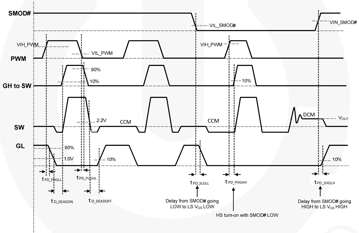
Figure 26. SMOD Timing Diagram
