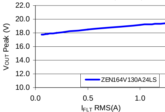
V_{OUT} Peak Vs I_{FLT} RMS ( I_{OUT} = 0 )
