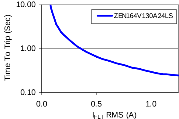
Time to Trip Vs I_{FLT} RMS ( I_{OUT} = 0 )
