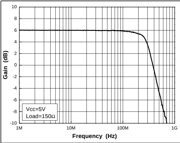
Figure 1. Frequency response
