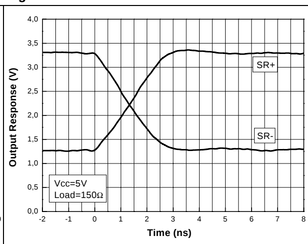
Figure 12. Slew rate
