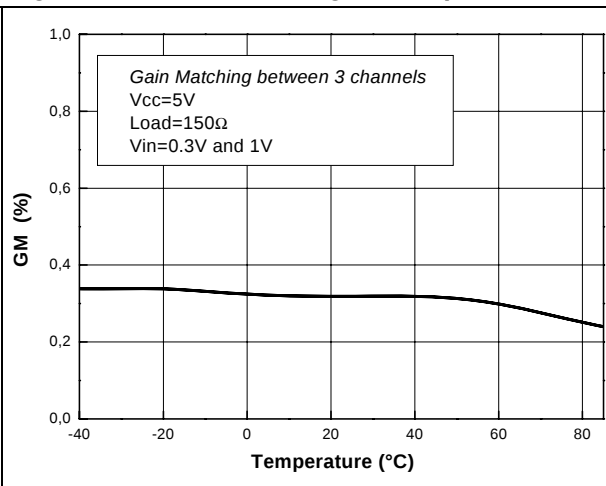
Figure 20. Gain matching vs. temperature
