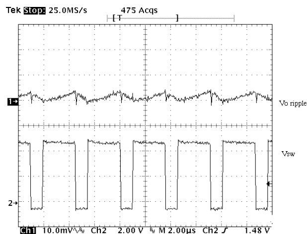
Figure 14. The Output Voltage Ripple Using One 100 \mu\text{F} POSCAP Capacitor
