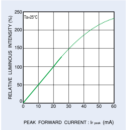
Relative Luminous Intensity - Forward Current
