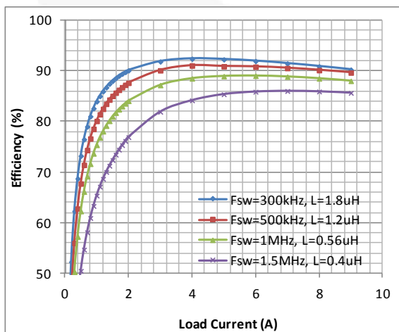
Figure 10. FAN233SV06P Efficiency vs. Load Current with V_{IN}=12\text{ V} and V_{OUT}=1.2\text{ V}
