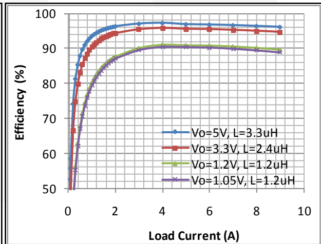
Figure 9. FAN233SV06P Efficiency vs. Load Current V_{IN}=12\text{ V} and f_{SW}=500\text{ kHz}
