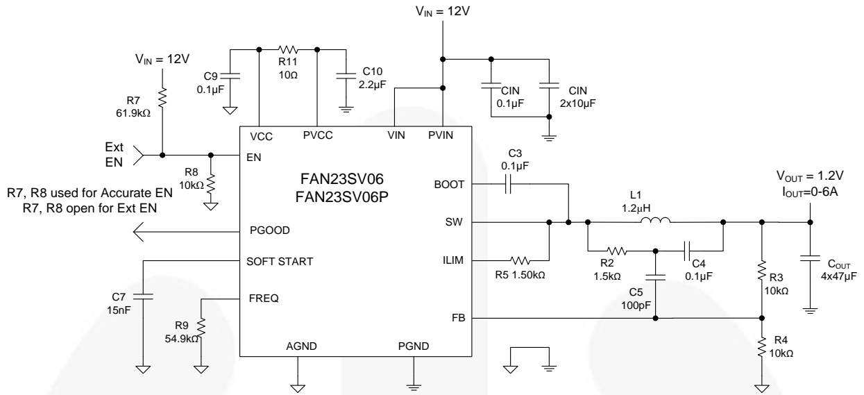
Figure 1. Typical Application with V_{IN} = 12\text{ V}
