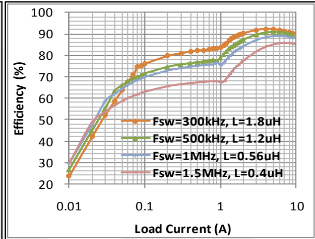
Figure 7. FAN233SV06 Efficiency vs. Load Current with V_{IN}=12\text{ V} and V_{OUT}=1.2\text{ V}
