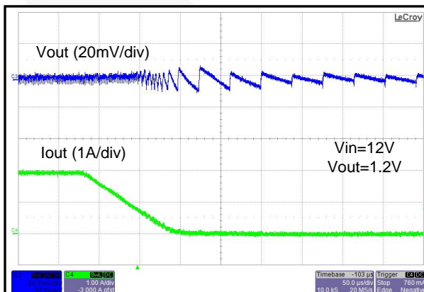
Figure 22. FAN23SV06 Operation as Load Changes from 2 A to 0 A
