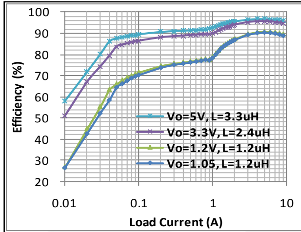
Figure 6. FAN233SV06 Efficiency vs. Load Current with V_{IN}=12\text{ V} and f_{SW}=500\text{ kHz}
