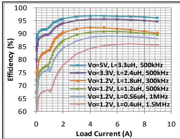
Figure 8. FAN233SV06 Efficiency vs. Load Current with V_{IN}=12\text{ V}
