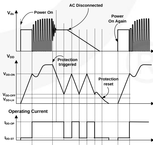
Figure 34. Latch Mode Operation
