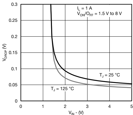
V_{DROP} vs. V_{IN} at I_L = 1 A
