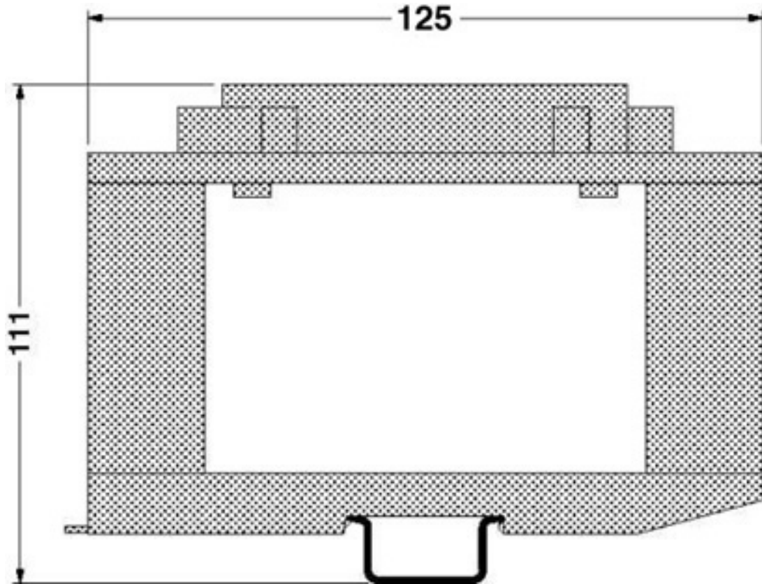
Dimensioned drawing
