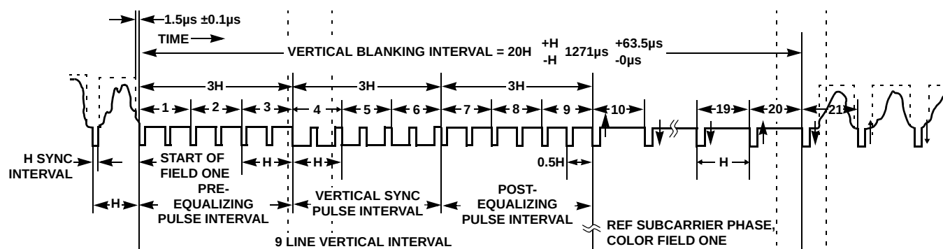
SIGNAL 1a. COMPOSITE VIDEO INPUT, FIELD ONE
