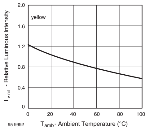
Figure 8. Rel. Luminous Intensity vs. Ambient Temperature
