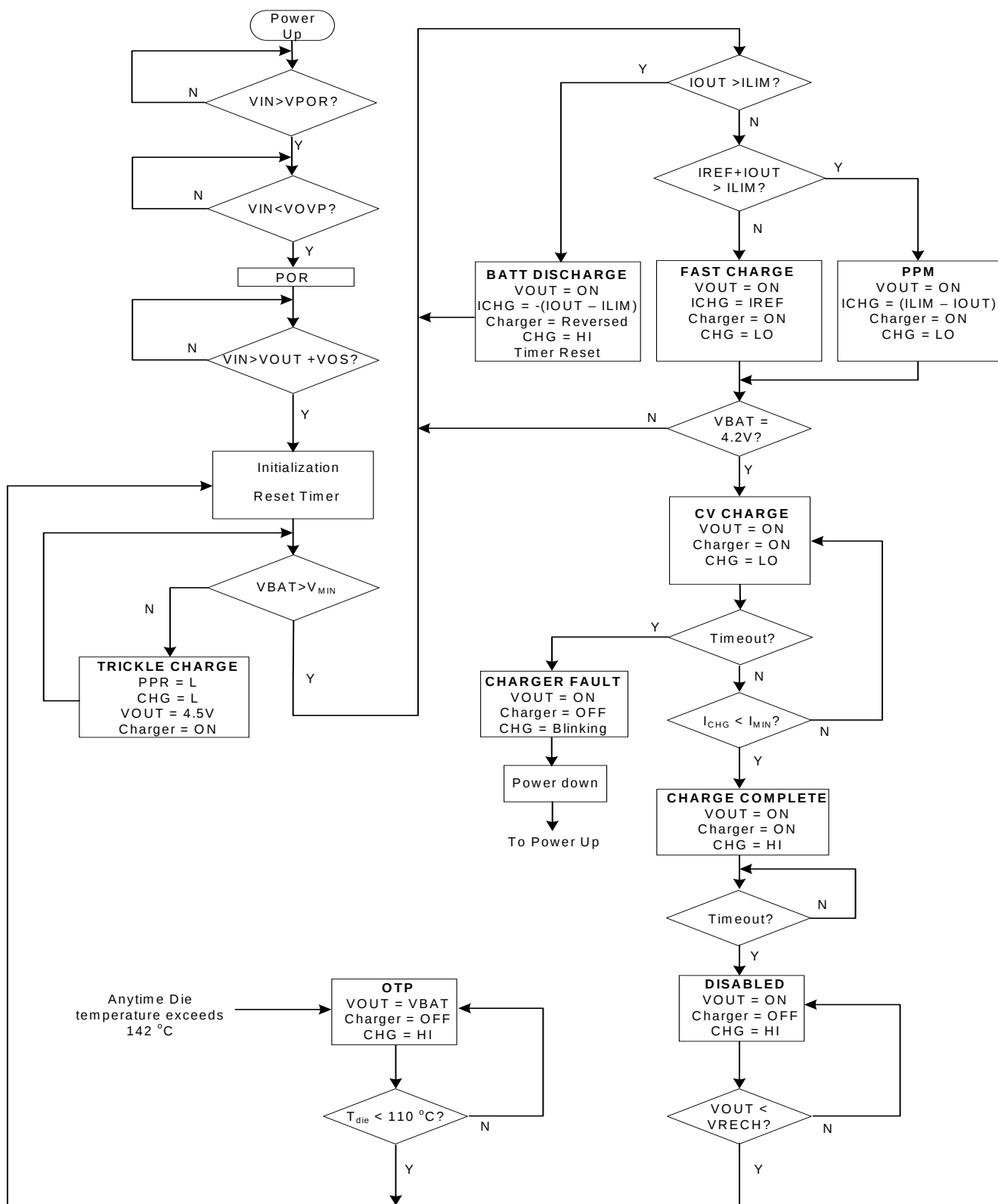
FIGURE 6. STATE DIAGRAM
