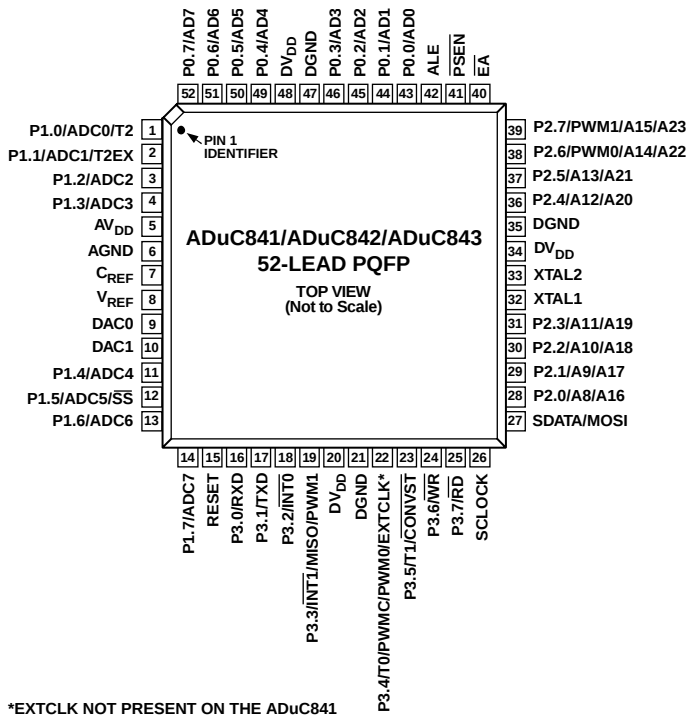
Figure 3. 52-Lead PQFP
