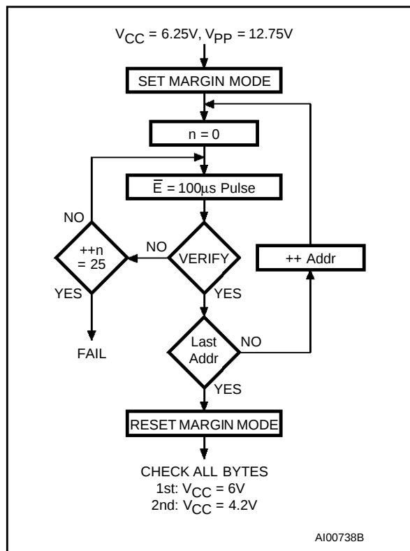
Figure 8. Programming Flowchart
