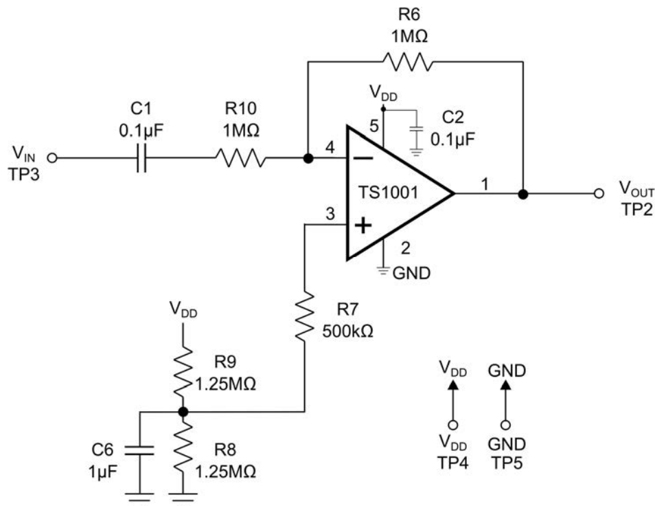
Figure 2. Inverting Configuration
