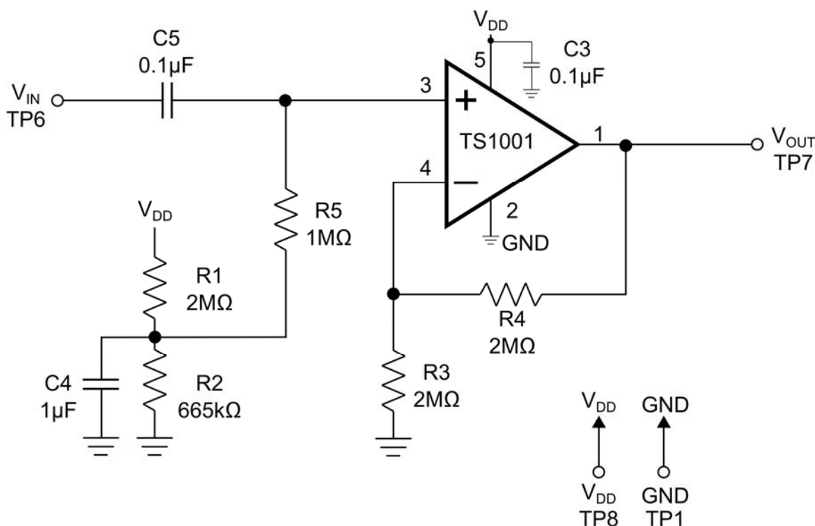
Figure 1. Non-Inverting Configuration
