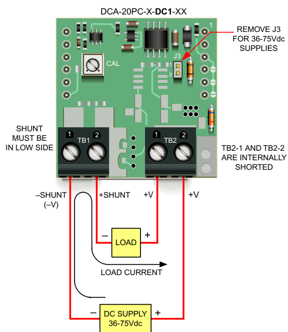
Figure 3. Low-Side Shunt Connections for "-DC1" Models Modified for 36-75Vdc Non-Isolated Power (See Technical Note 6)
