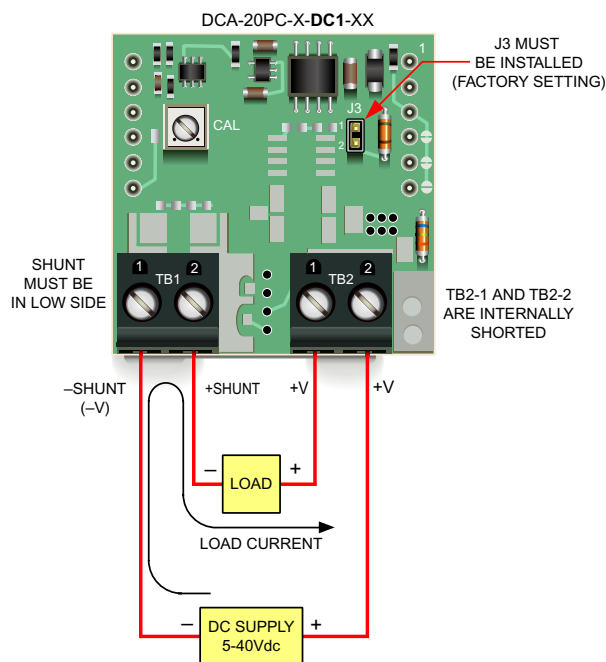
Figure 2. Low-Side Shunt Connections for "-DC1" 5-40Vdc Non-Isolated Supply Models
