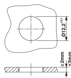
Panel cutout
