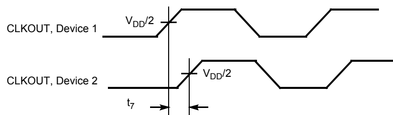
Figure 9. Device-Device Skew
