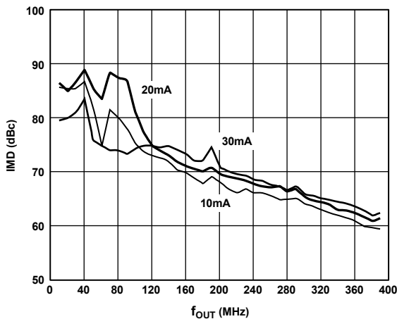
Figure 25. AD9788 IMD Performance vs. Full-Scale Output Current, 4x Interpolation, f_{DATA} = 200 MSPS
