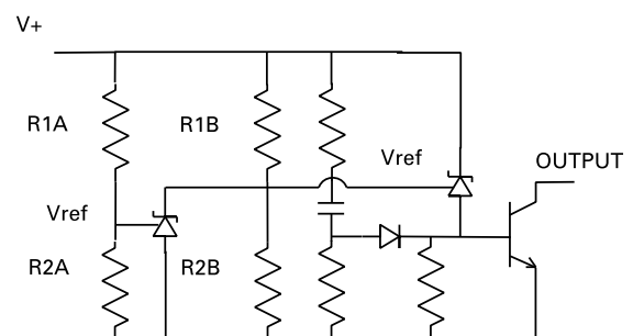
SERIES REGULATOR
