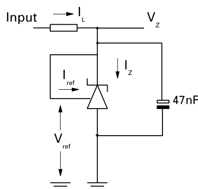
Fig 1 - Test Circuit for V_Z = V_{ref}
