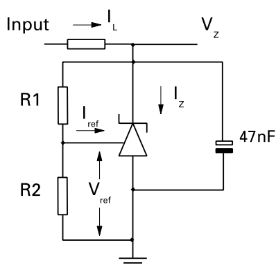
Fig 2 - Test Circuit for V_Z > V_{ref}
