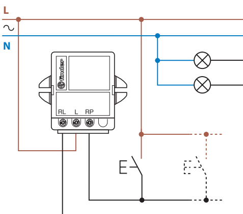
Type 15.51 - 4 wire connection
