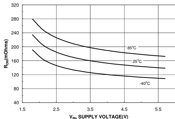
Figure 9. R_{ON} vs. Input Voltage
