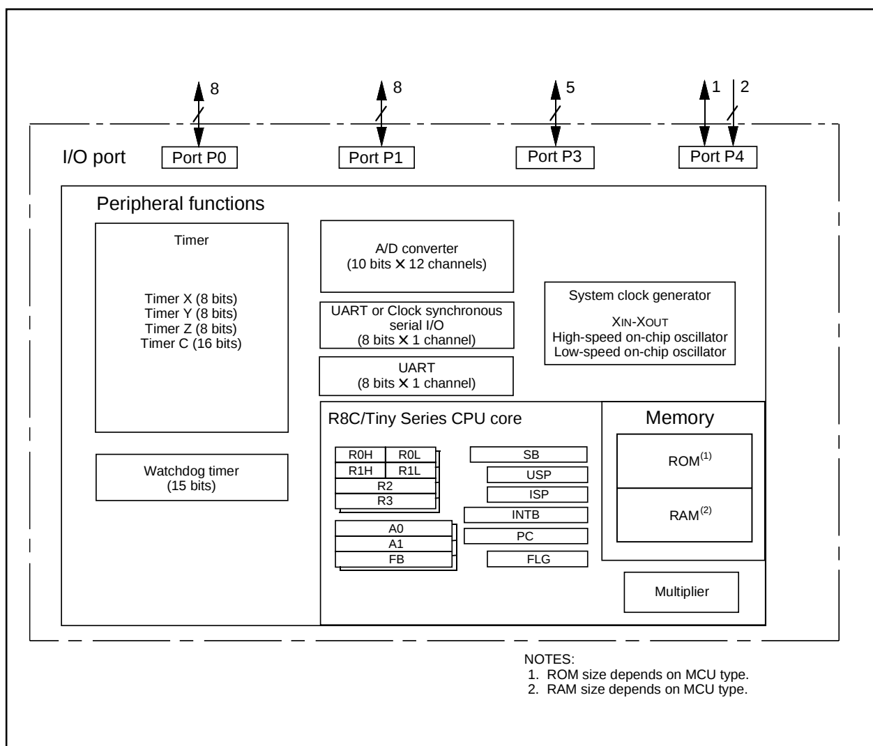
Figure 1.1 Block Diagram
