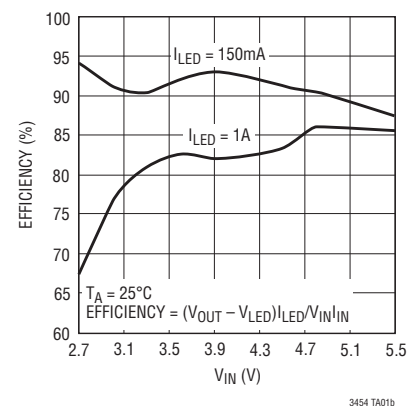
LED Power Efficiency vs V_{IN}
