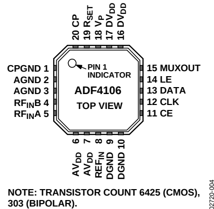
Figure 4. 20-Lead LFCSP_VQ Pin Configuration
